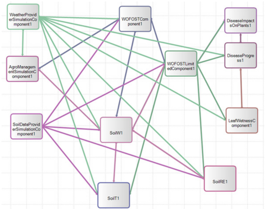
Figure 3 Wofost - Connections between all components (including optional components)
