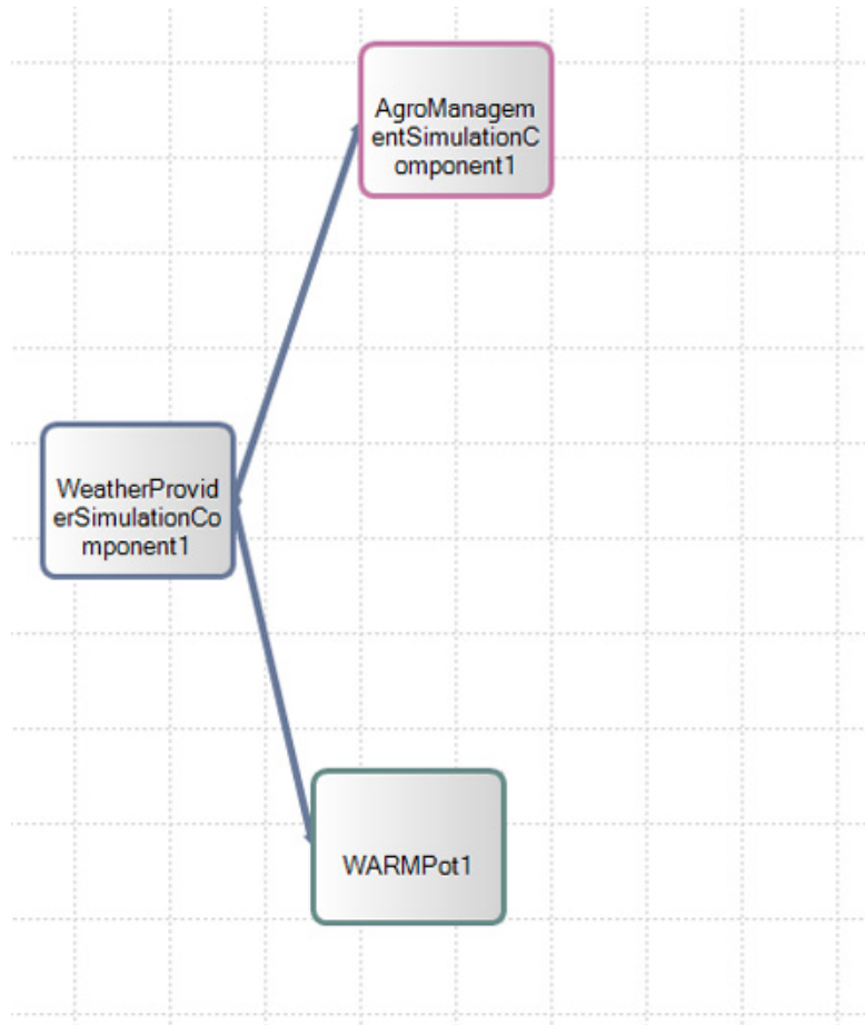
Figure 2 WARM - Connections between mandatory components
